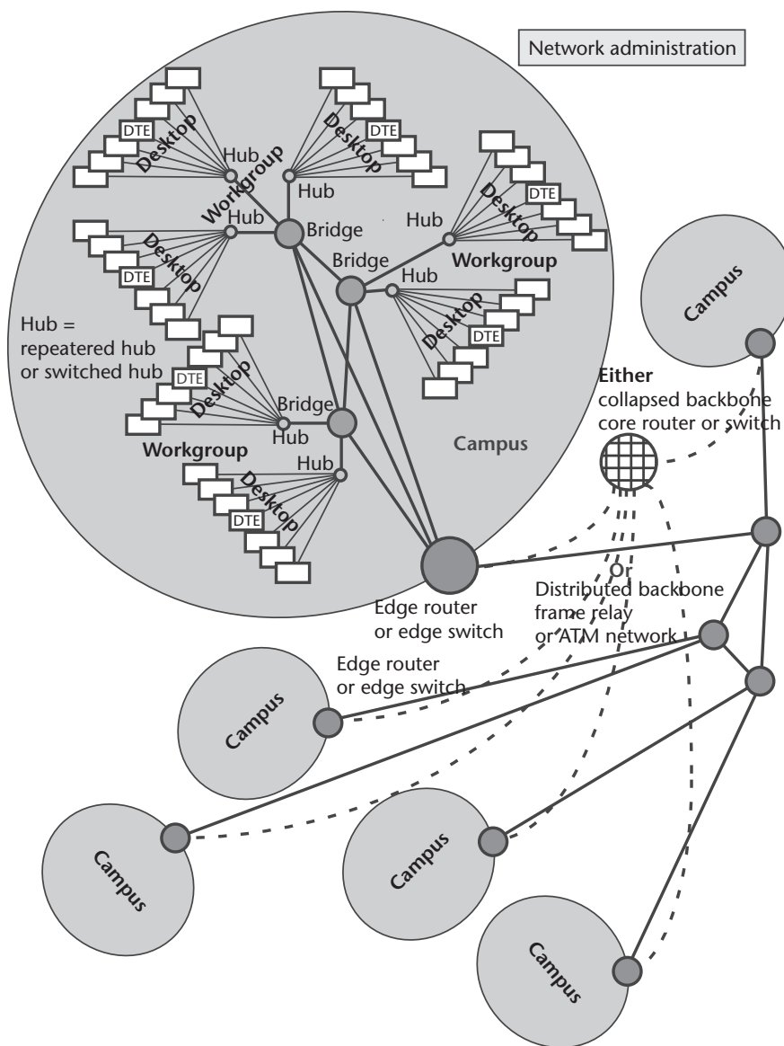
Figure 6.1 Enterprise catenet.
