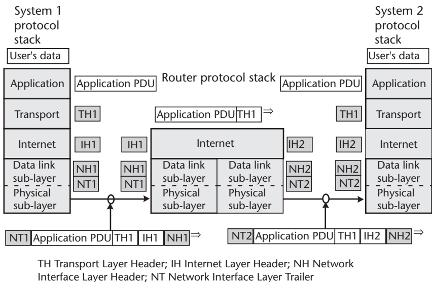
Figure 5.3 Headers/trailers employed in host–router–host path.
