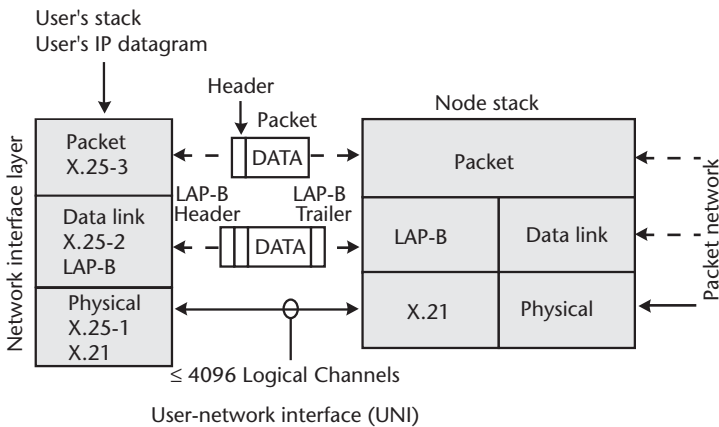
Figure 4.3 X.25 architecture.
