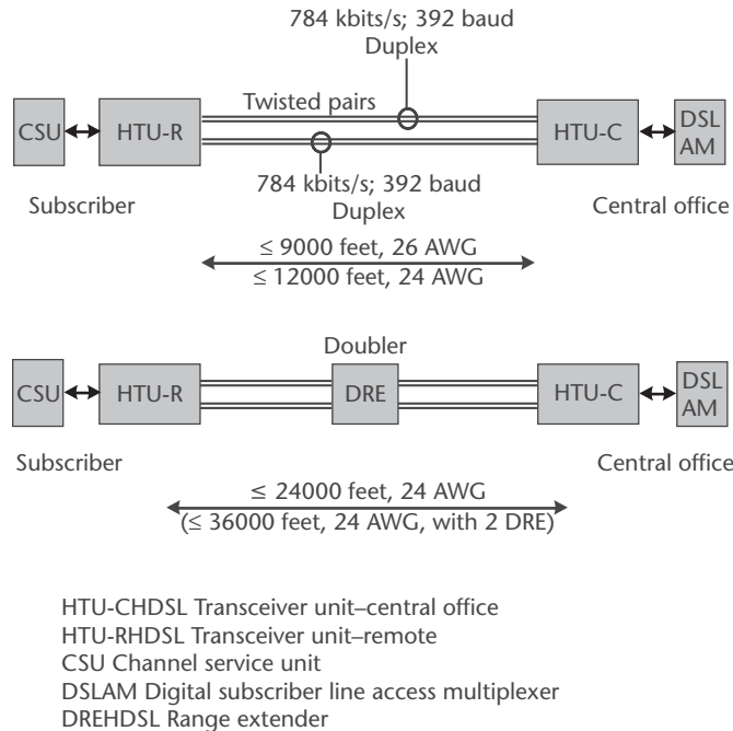
Figure 8.4 HDSL implementation.
