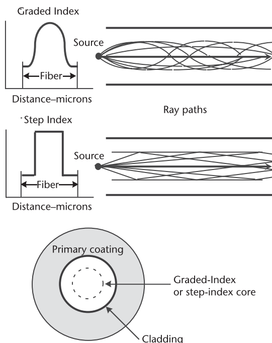
Figure 7.10 Short-distance fibers.
