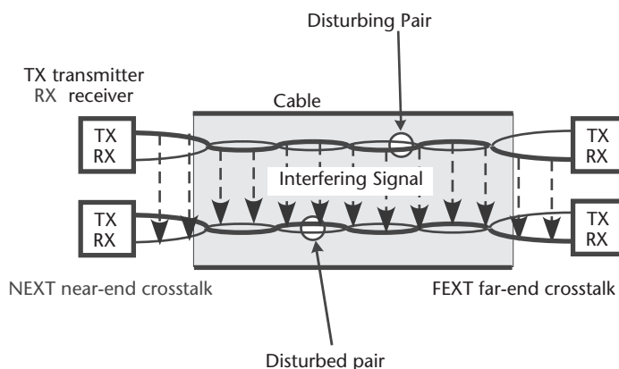
Figure 7.4 Crosstalk components.
