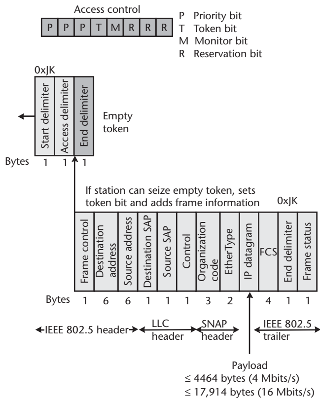
Figure 3.11 Token Ring frame.
