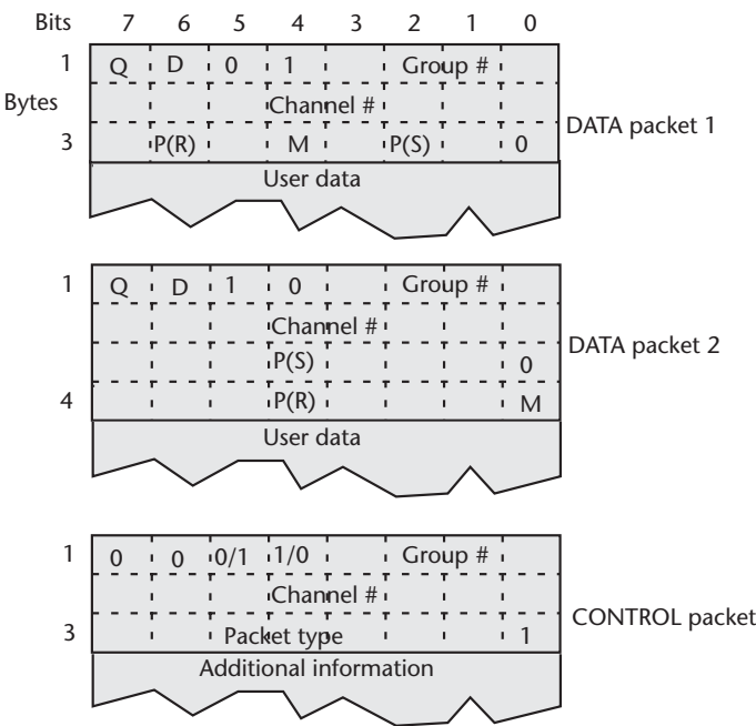
Figure 4.4 Packet formats.
