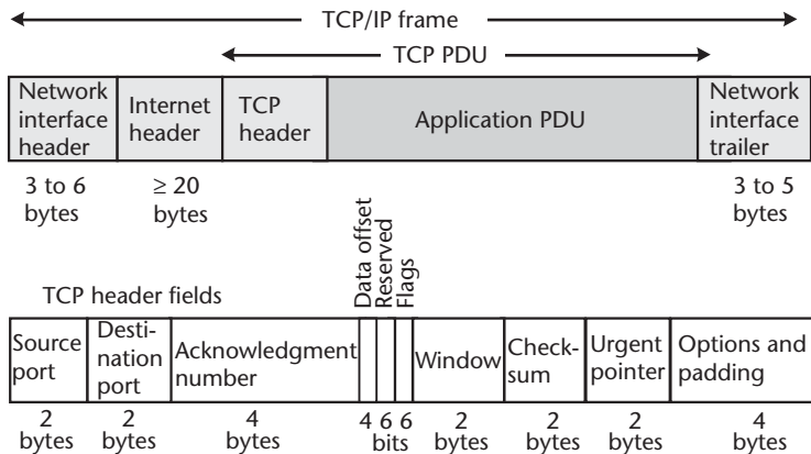
Figure 1.3 TCP header and TCP/IP frame.
